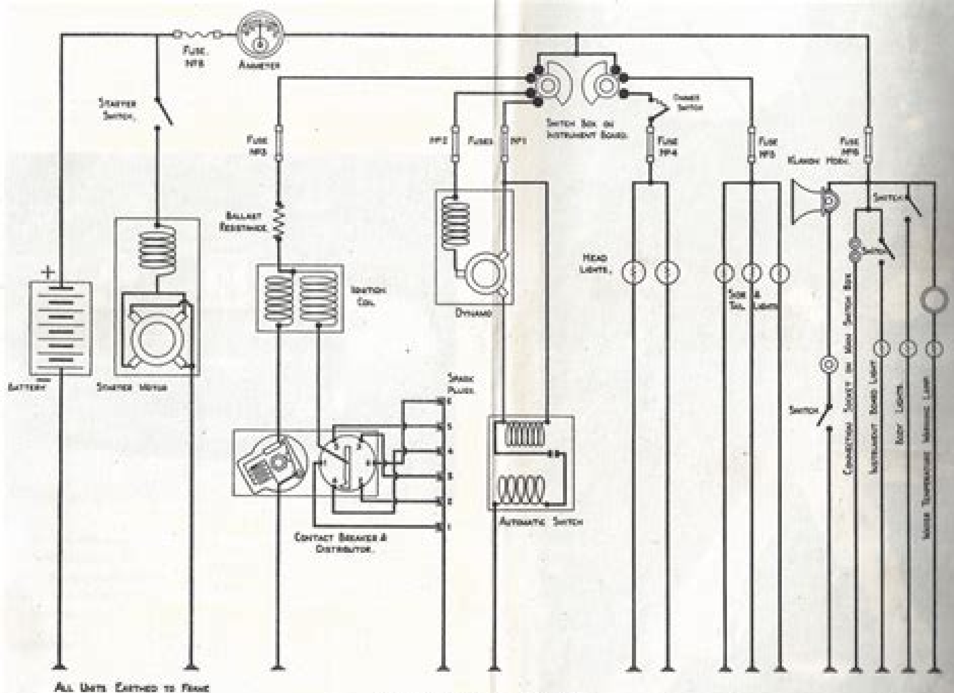
FIG. 5. TECHNICAL WIRING DIAGRAM. (SOME OF THE SWITCHES)
