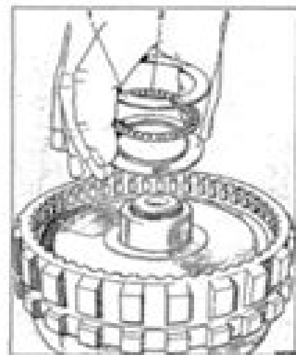
Fig. 11B-16 Fitting the steel and thrust bearing to the outer face of the rear internal gear 1. 5/16 flanged nut 2. Thrust bearing 3. 1/2 flanged nut
