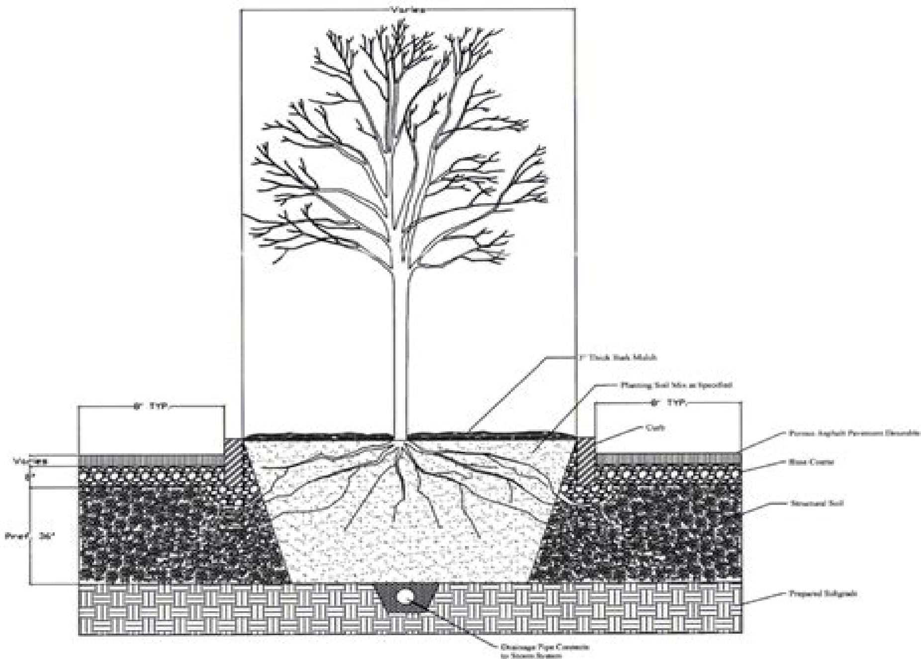
BARE ROOT TREE IN TYPICAL PARKING LOT ISLAND
