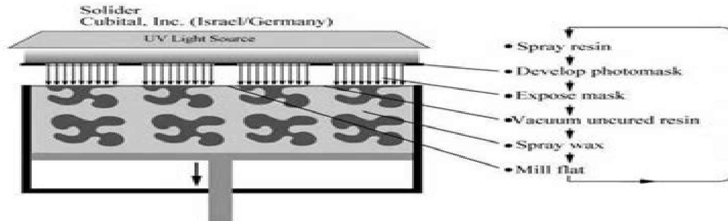
Fig. Solid Ground Curing Process.
