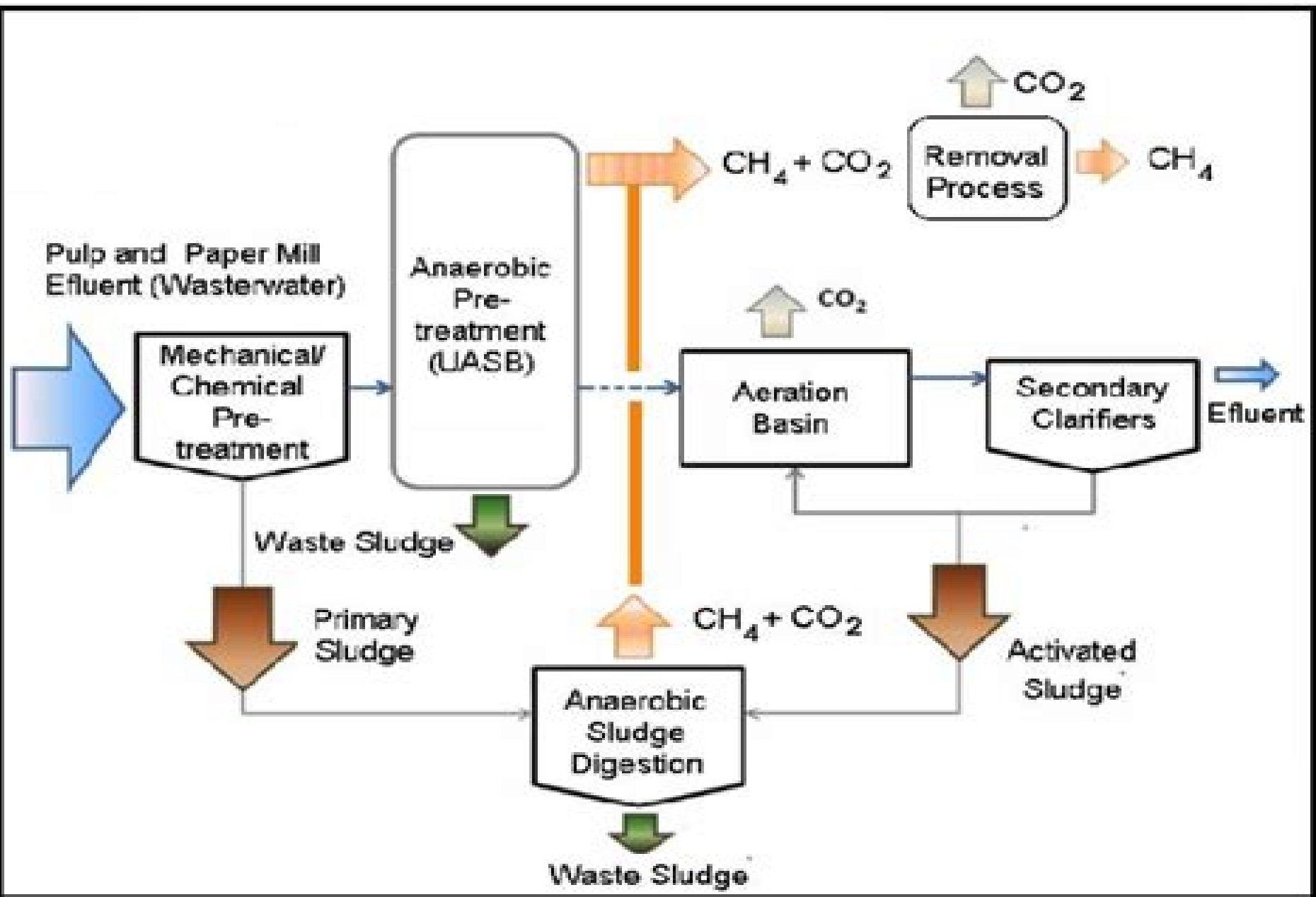
Figure 1. Wastewater treatment of pulp and paper mill effluent
