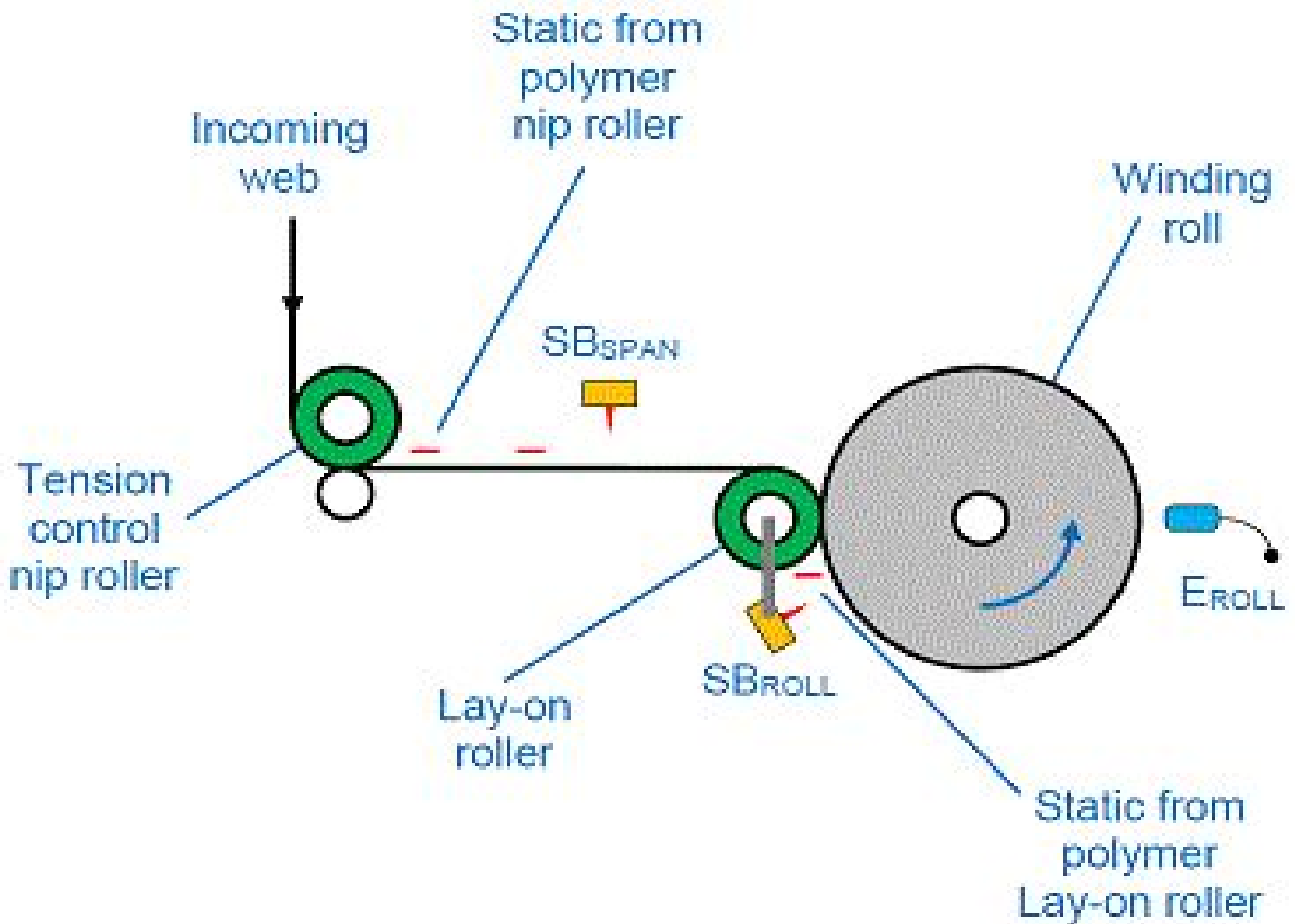
Figure 2: Static bar SB_{SPAN} dissipates static from the polymer nip roller and SB_{ROLL} dissipates static from the lay-on roller.
