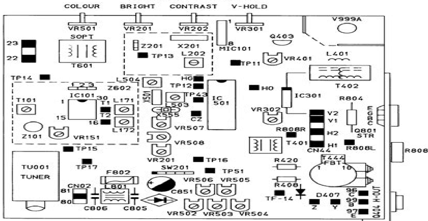
PARTS LOCATION DIAGRAM
