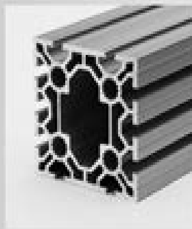
Heavy duty extrusion 100x100
