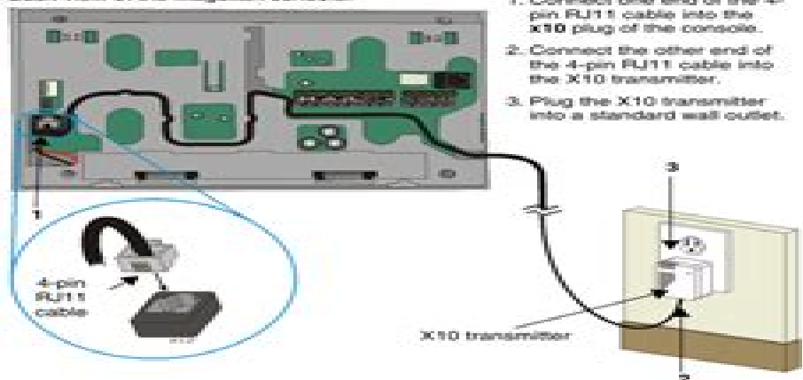
Figure 9: Connecting the X10 Transmitter
