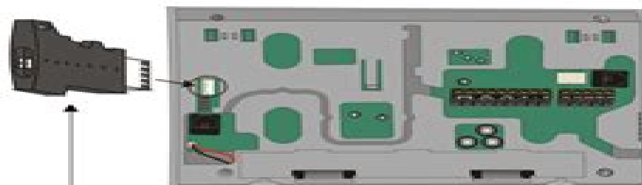
Figure 10: Connecting a Paradox Memory Key (PMC-3)
