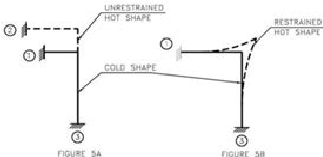
FIGURE 5 – RESTRAINED PIPING SYSTEM
