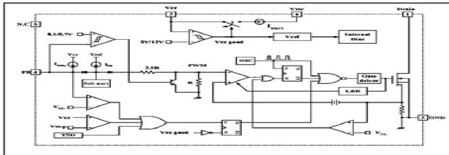
Figure 2. Functional Block Diagram of FSDM0565RB
