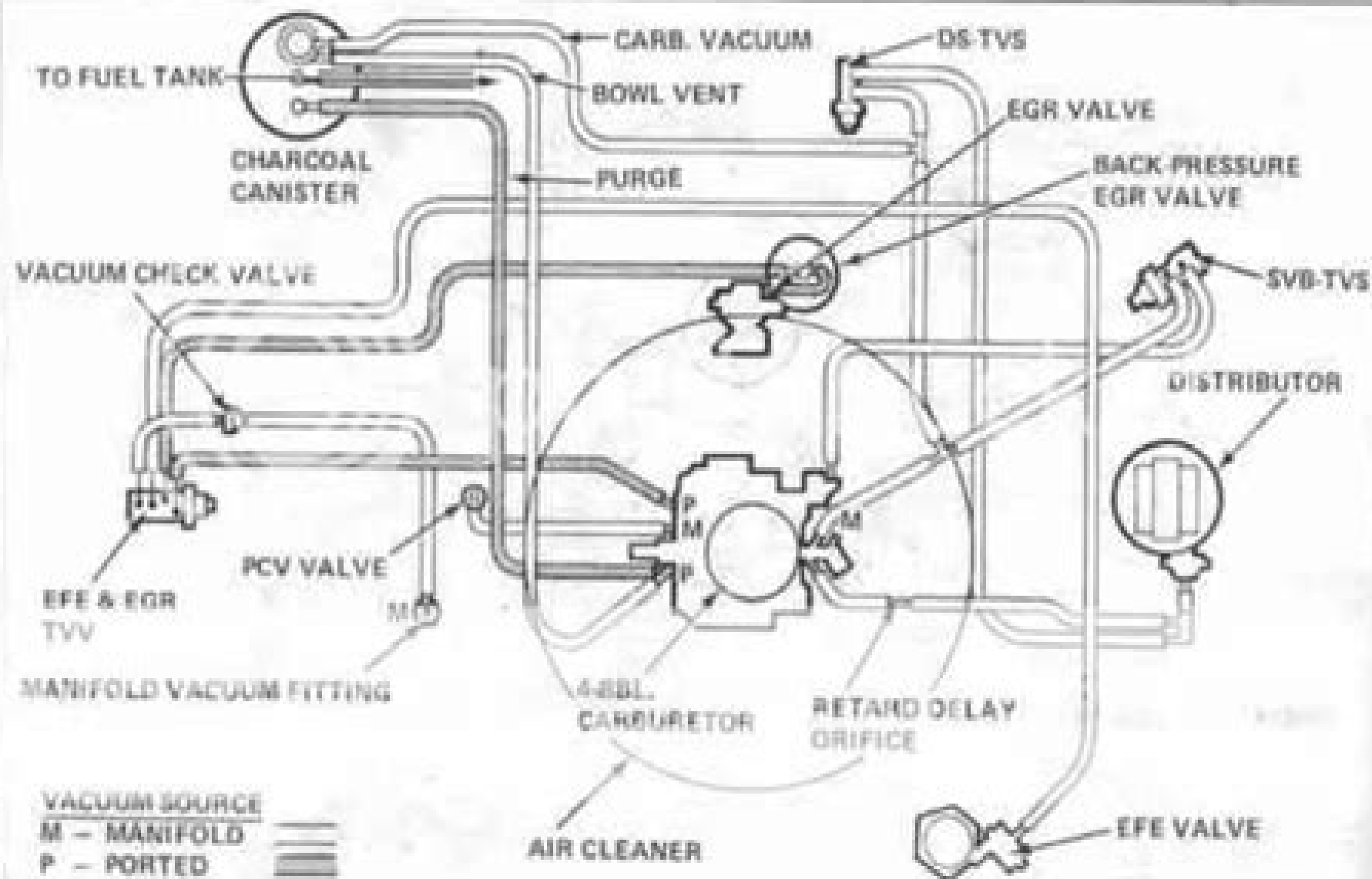
Fig. 6E-29 V8-400 4 BBL VIN Code Z (Auto Trans., Dual Exhaust)
