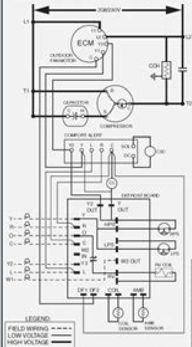
Figure 15. Wiring Diagram for 2, 4, & 5 Ton Premium / Ultra Premium Models (FT4BF-048KA, PSH4BF-048KA)
