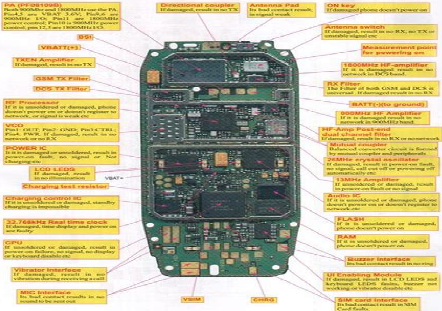
NOKIA 3310/3330 Mobile Phone Troubleshooting Locations 1
