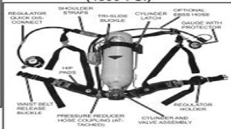
TYPICAL INDUSTRIAL SCBA 4500 PSI W/ OPTIONAL ACCESSORIES
