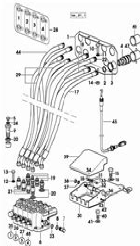
Section: ACCESSORIES REXROTH SILVER 110 6-WAY AUXILIARY CONTROL VALVE Ref.: SE.00.4
