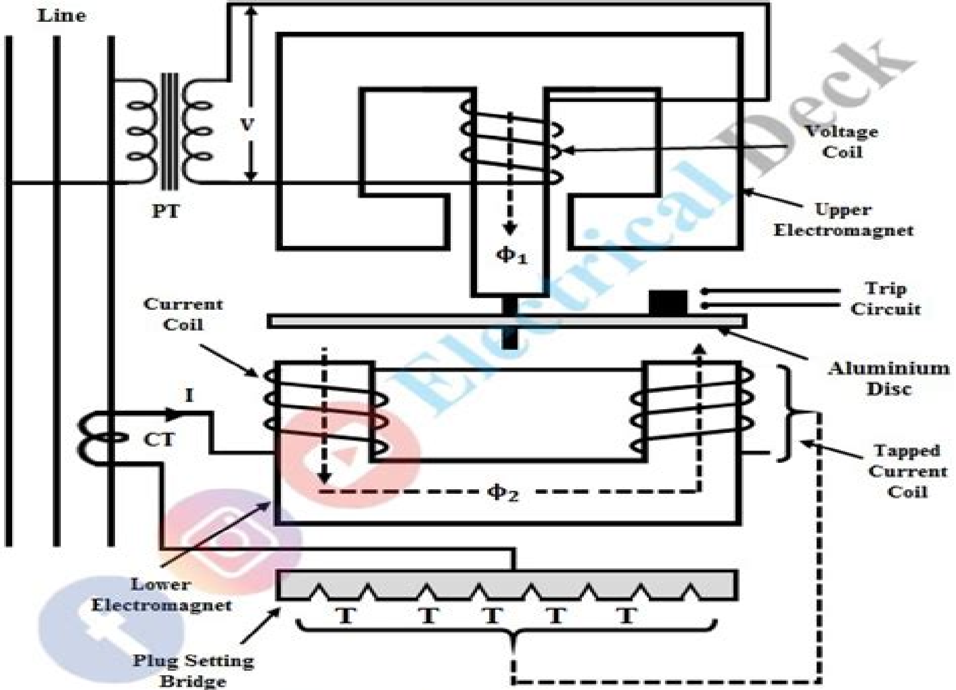
Reverse Power Relay
