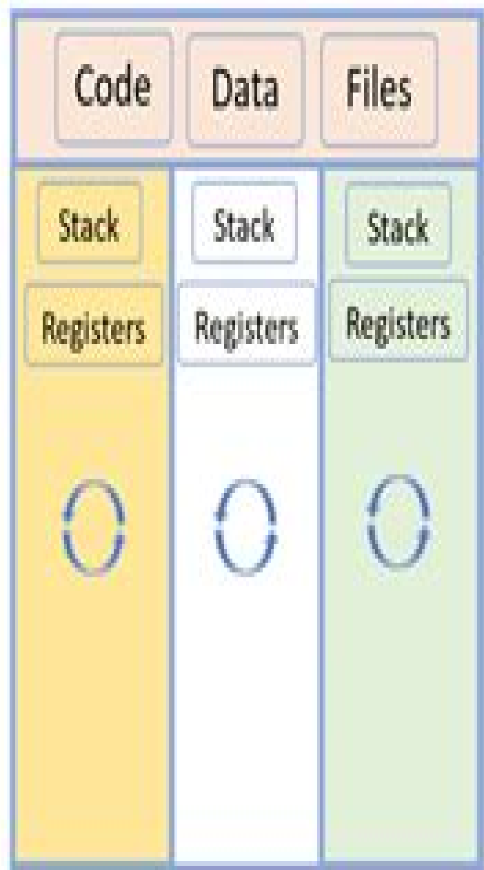
Multi Threaded Process
