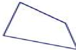
convex polygon
