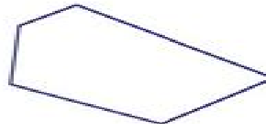
pentagon
