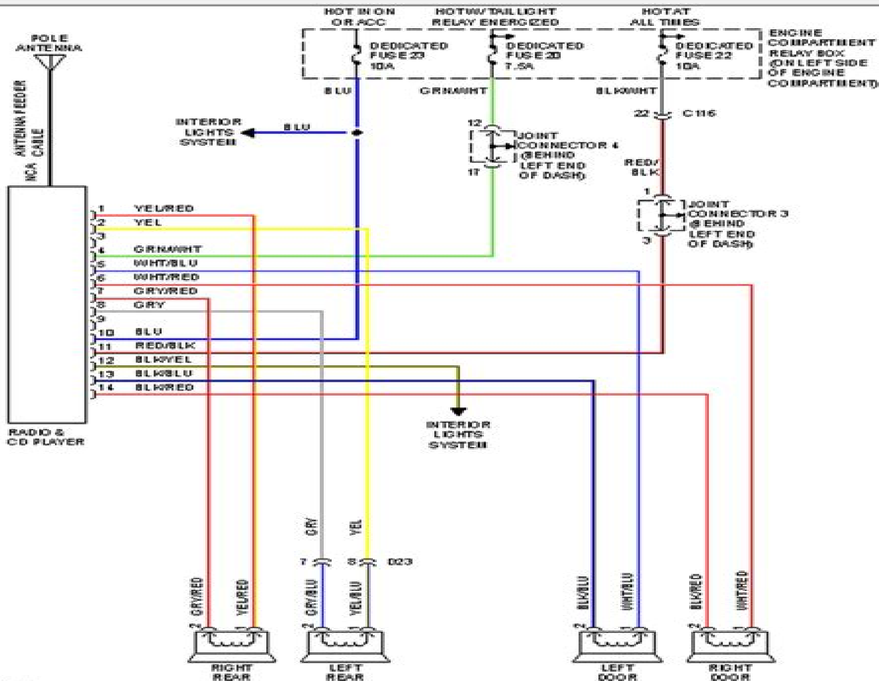
Fig. 39: Radio Circuit, W/O Amplifier
