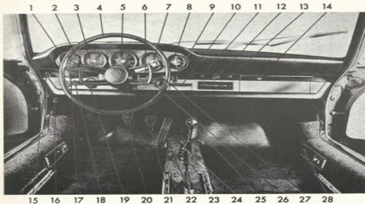
Instruments and Controls for left Hand steering
