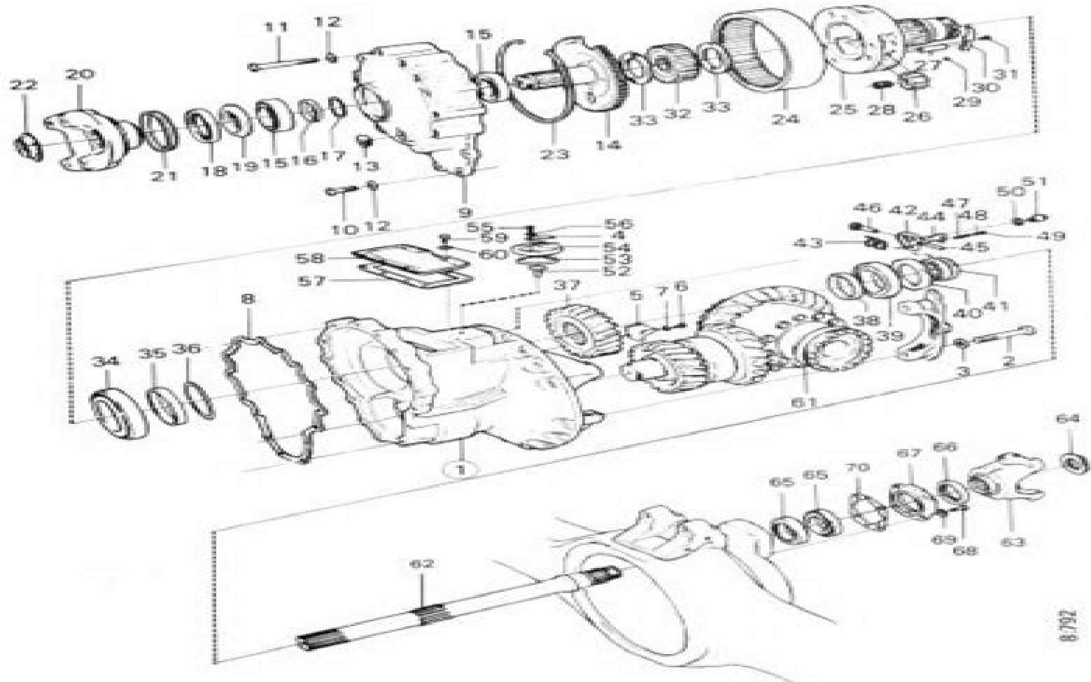
Axle gear RBP831, planetary gear
