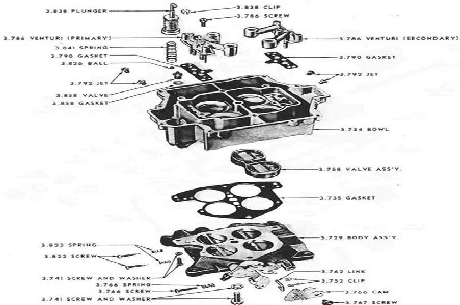
ROCHESTER CARBURETOR FLOAT BOWL AND THROTTLE BODY (1955 4 Barrel Type)
