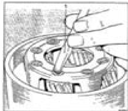
Fig. 718-14 Staking a piston pin 1. Oil
