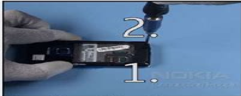
4. Remove both screws in the order shown.
