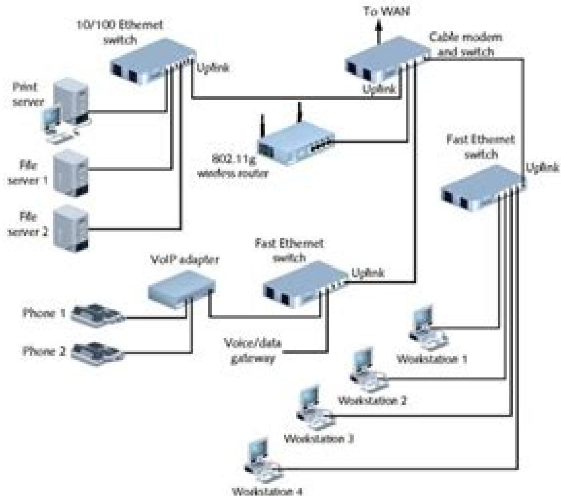
Figure 15-2 Wiring schematic
