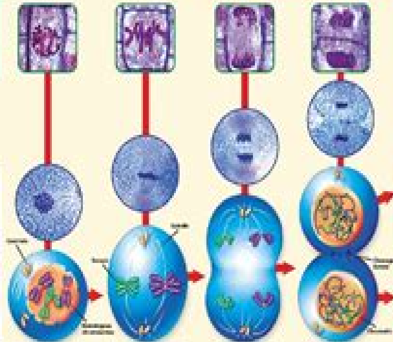
Prophase I
