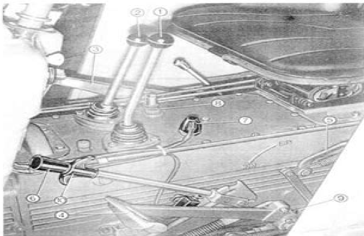
Fig. 2 Mechanical controls seen from the left
