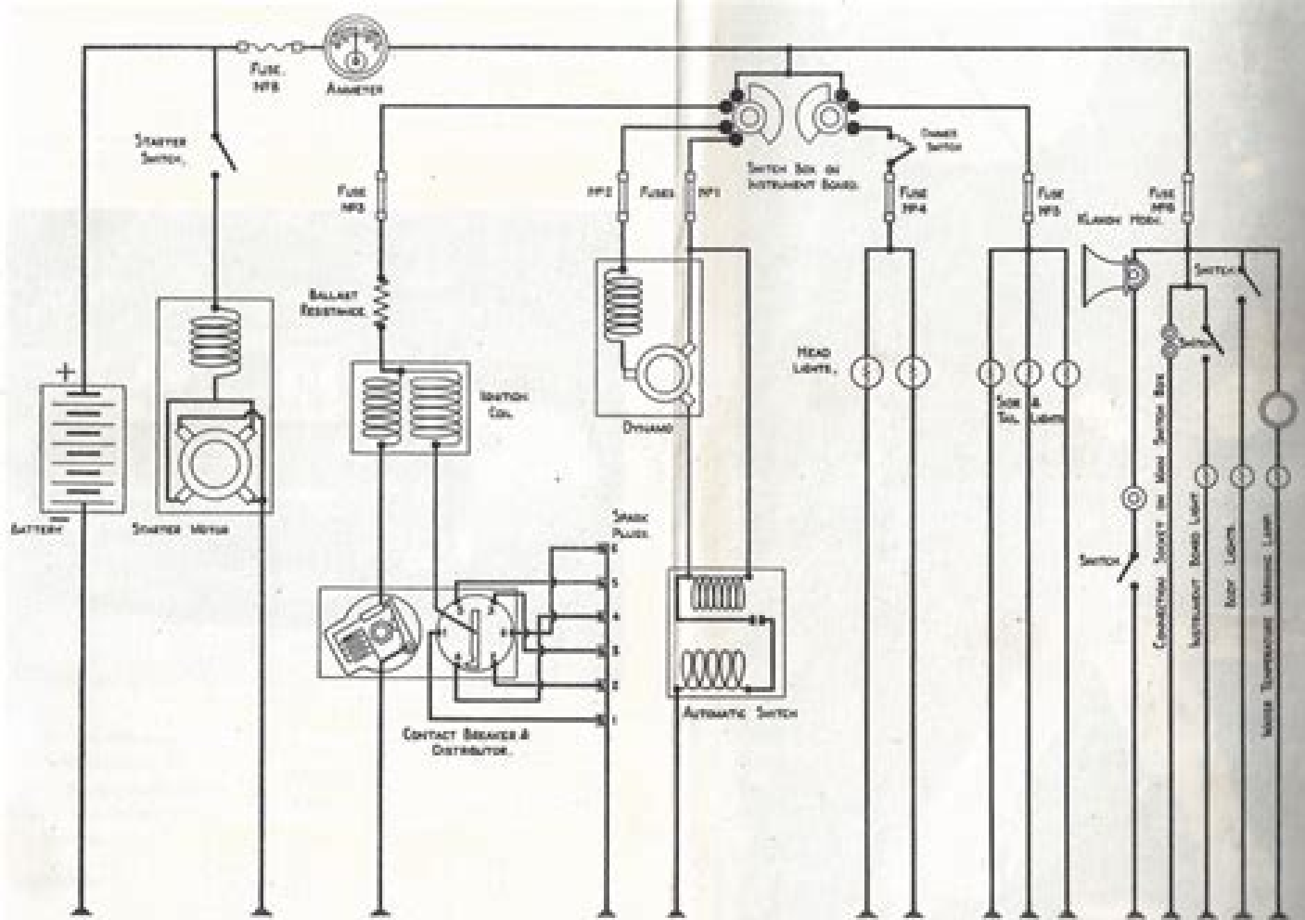
FIG. 5. TECHNICAL WIRING DIAGRAM. (SOME OF THE WIRING)
