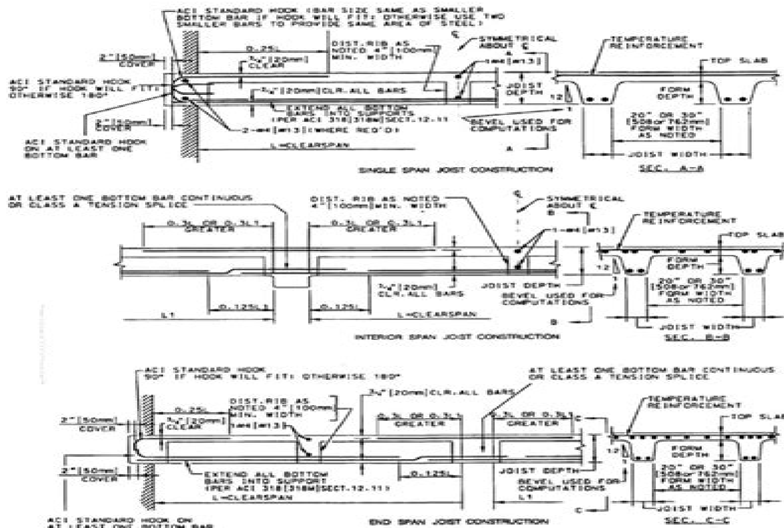
Fig. 3—Typical details for one-way joist construction.
