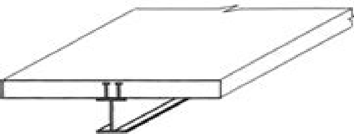
1. Solid composite beams
