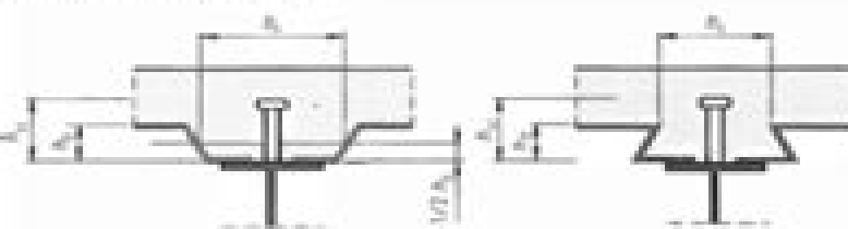
2. Beam with profiled steel sheeting parallel to the beam
