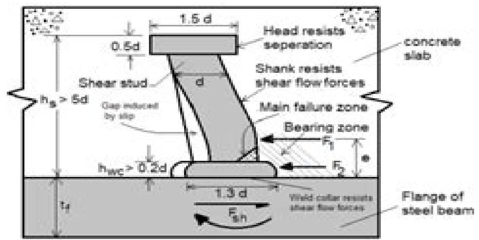
4. Dowel action of a stud shear connector
