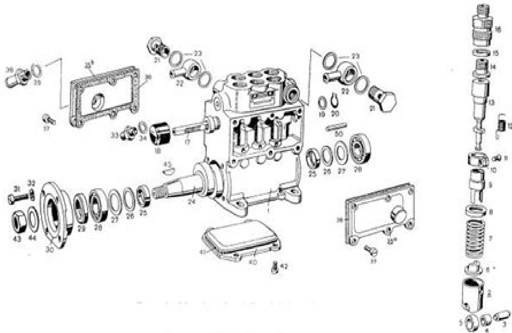
Pump
