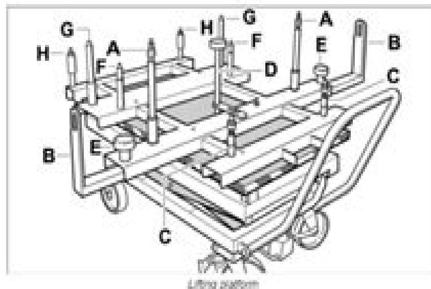
Lifting platform
