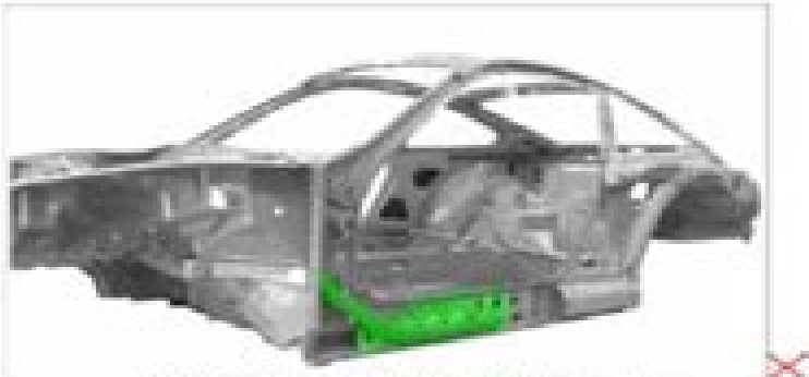
Installation position of lower side member reinforcement
