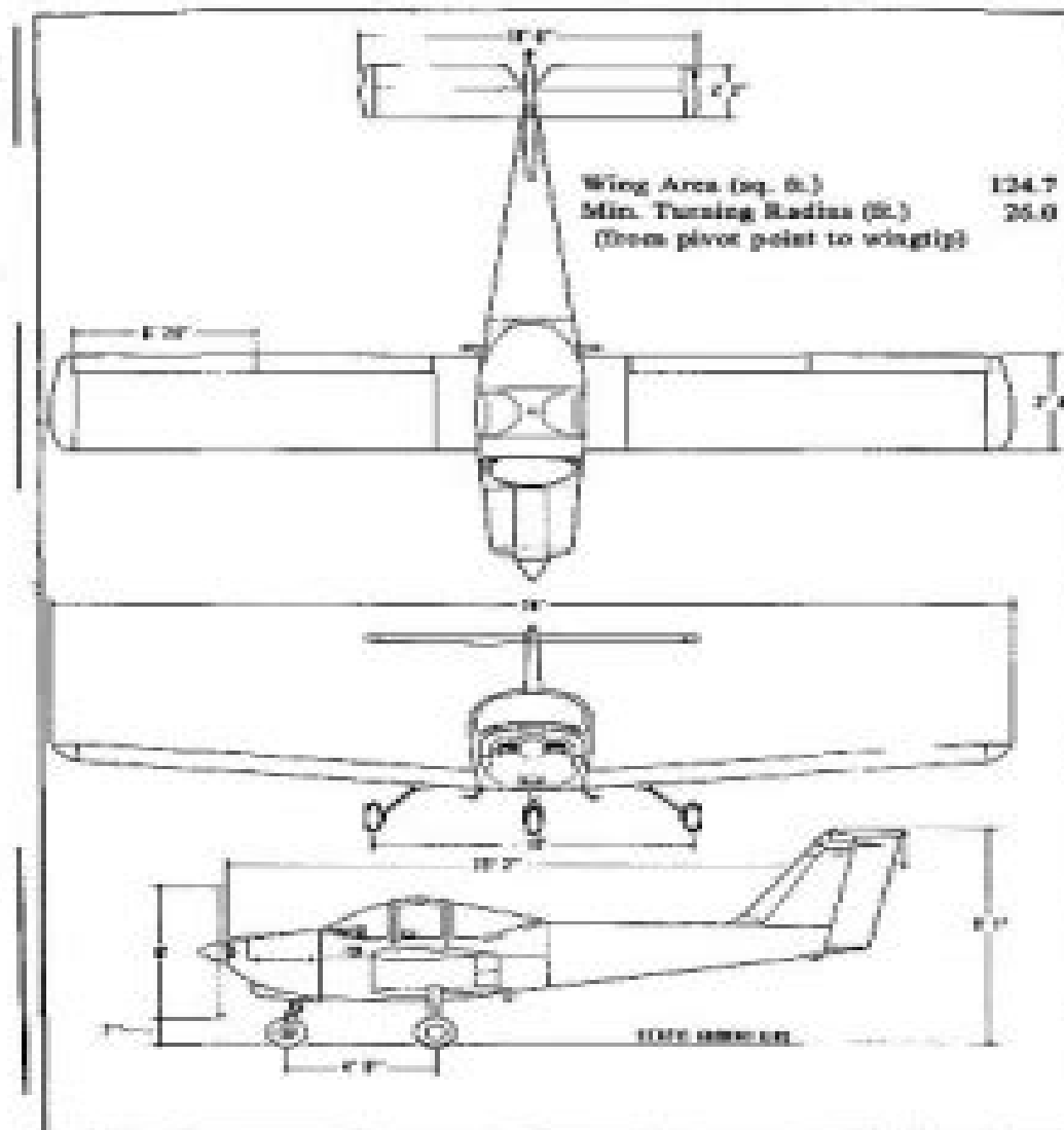
THREE VIEW Figure 1-1
