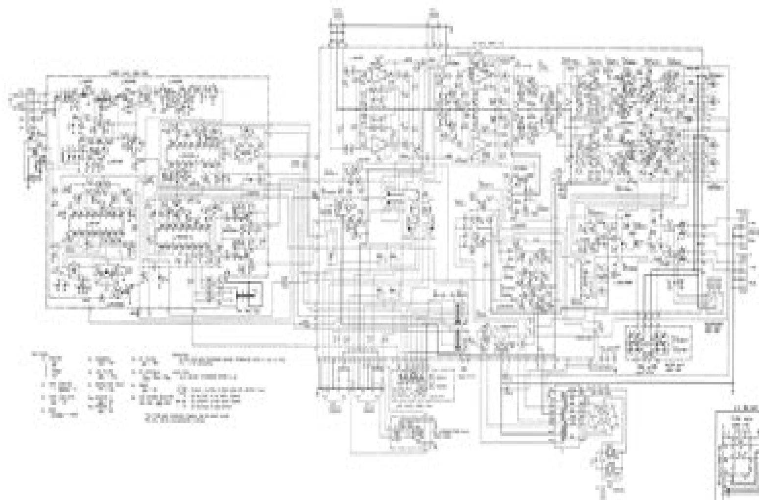
SCHEMATIC DIAGRAM FOR S, S/G TYPE
