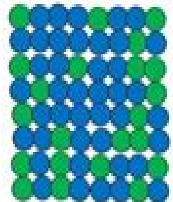
Solid solution
