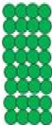
Conglomerate
