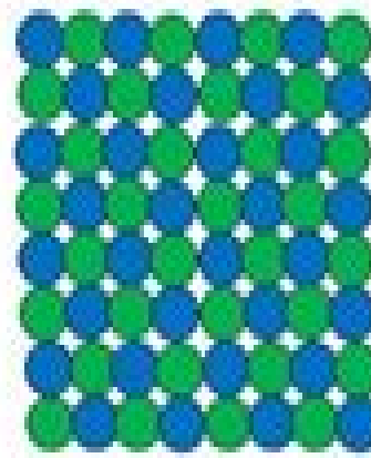
Racemic compound
