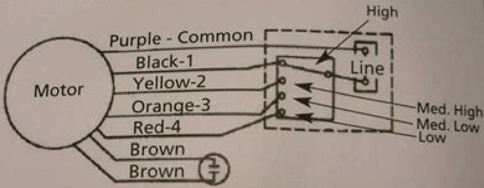
Figure 2 - Wiring Diagrams
