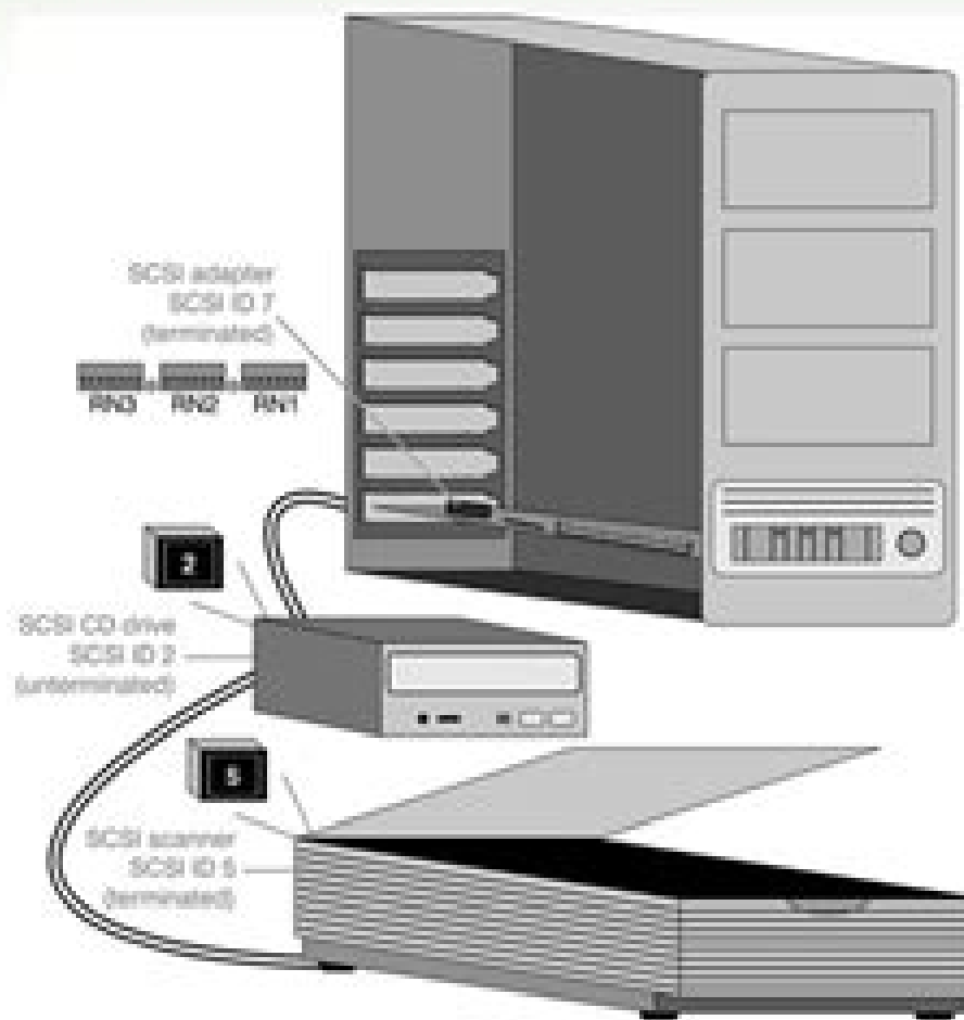
IDE/SCSI – Figure 7.34
