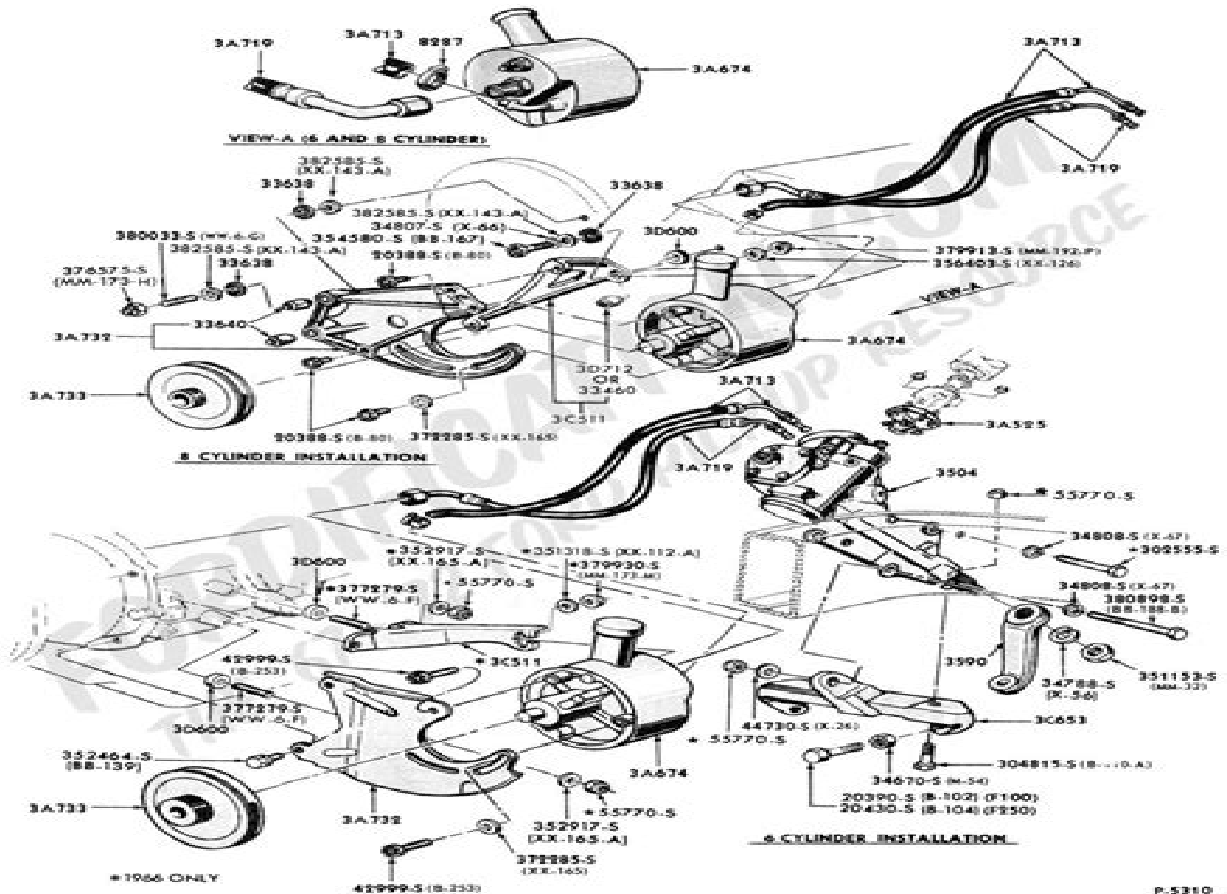
POWER STEERING SYSTEM 1966/68 F100/250 (4 x 2)
