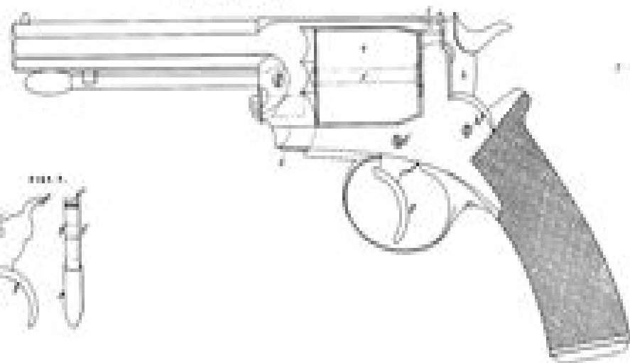
FIG. 1. Side View.
