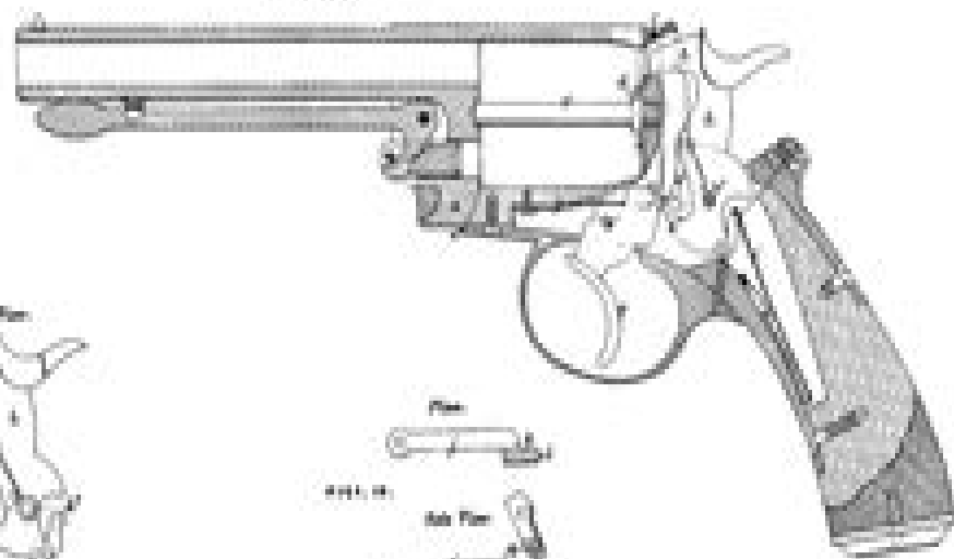
FIG. 3. Longitudinal Section.
