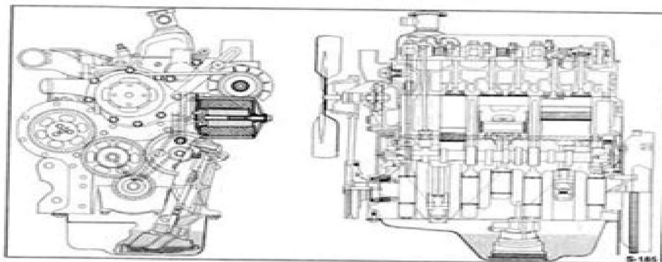
Figure 3 3-Cylinder Engine Lubrication System
