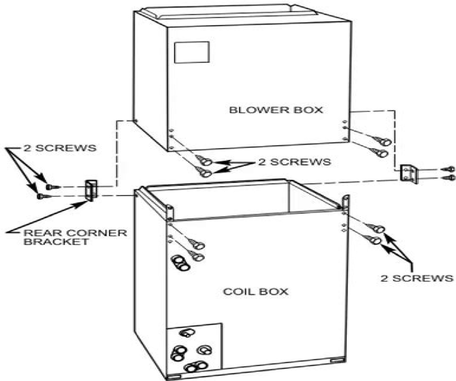
Fig. 5 – Modular Unit Assembly
