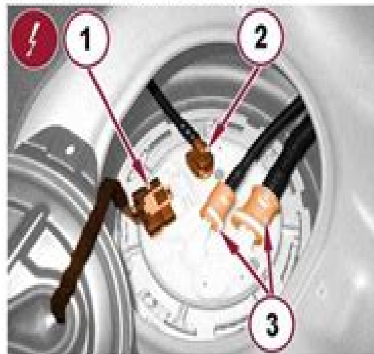
Fig 4: Connector, Fuel Delivery Pipe &amp; Fuel Vapor Pipe Quick Coupling
