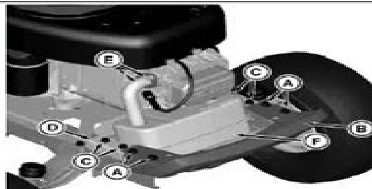
A—Cap Screw B—Hood Pivot Bracket C—Cap Screw D—Heat Shield
