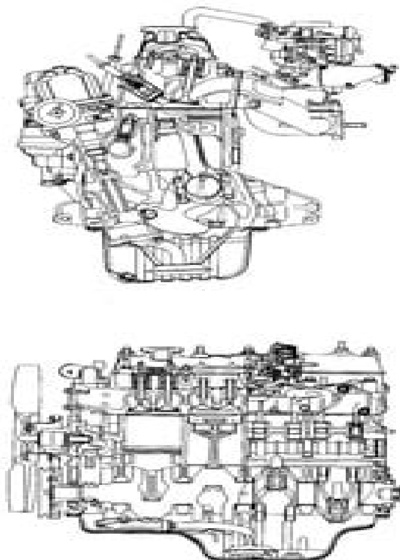
40' Engine Sectional View
