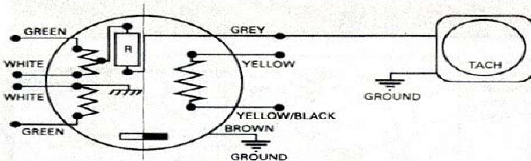
WIRING DIAGRAM FOR TACH Single or Dual DUCATI
