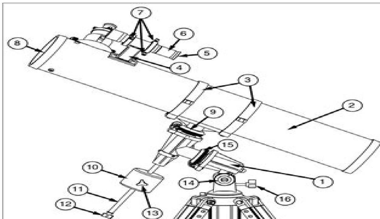
Fig. 2a: The Meade Model 4504 4.5" Equatorial Reflecting Telescope.
