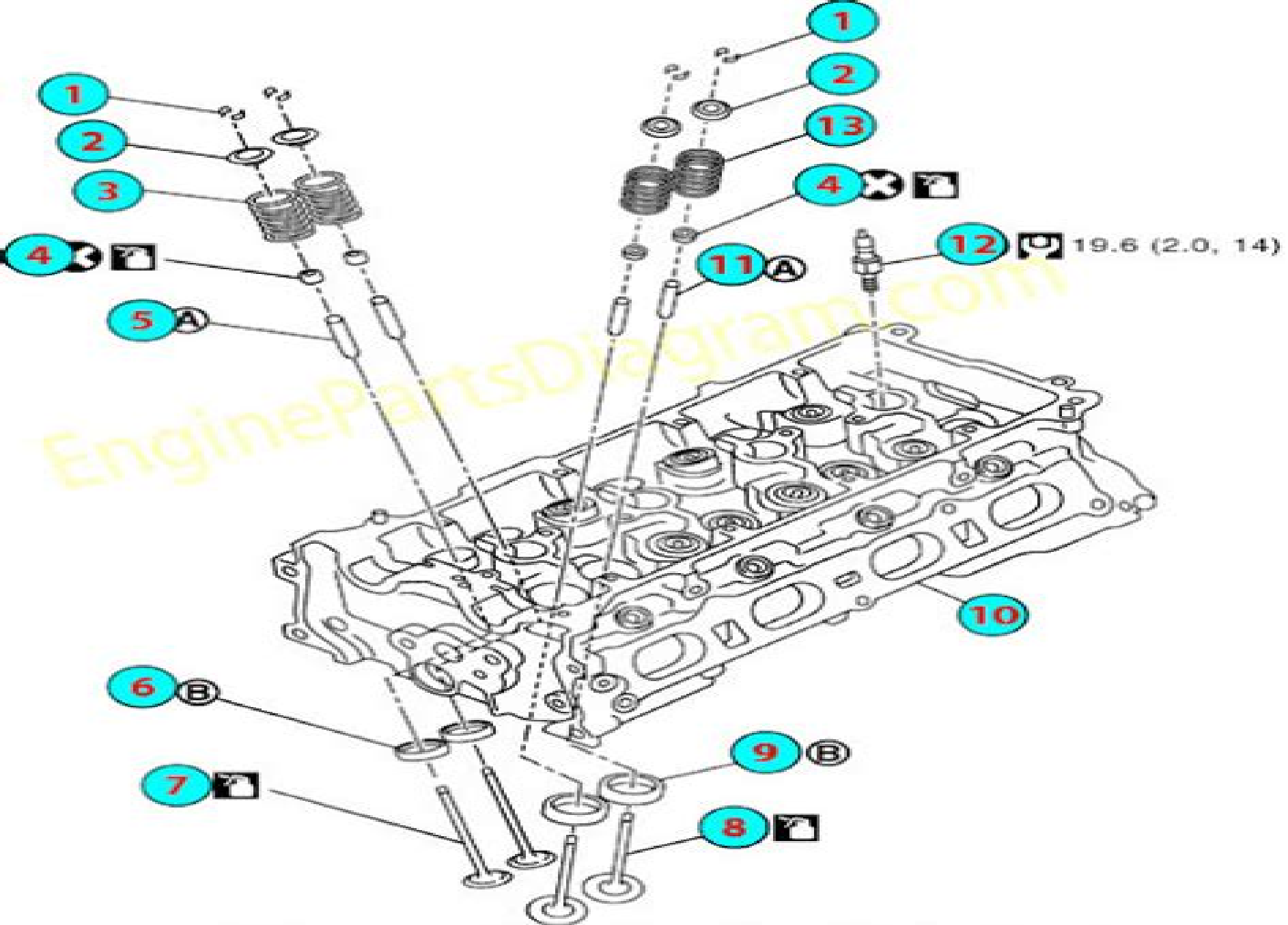
2007-2013 Nissan X-Trail Petrol Engine Cylinder Head Diagram
