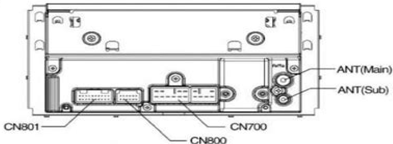
CN801 20P Connector
